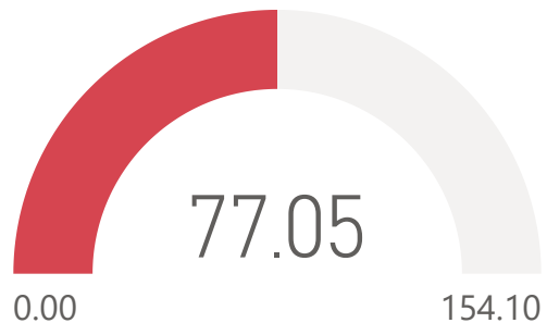
Service_Quality_Score
